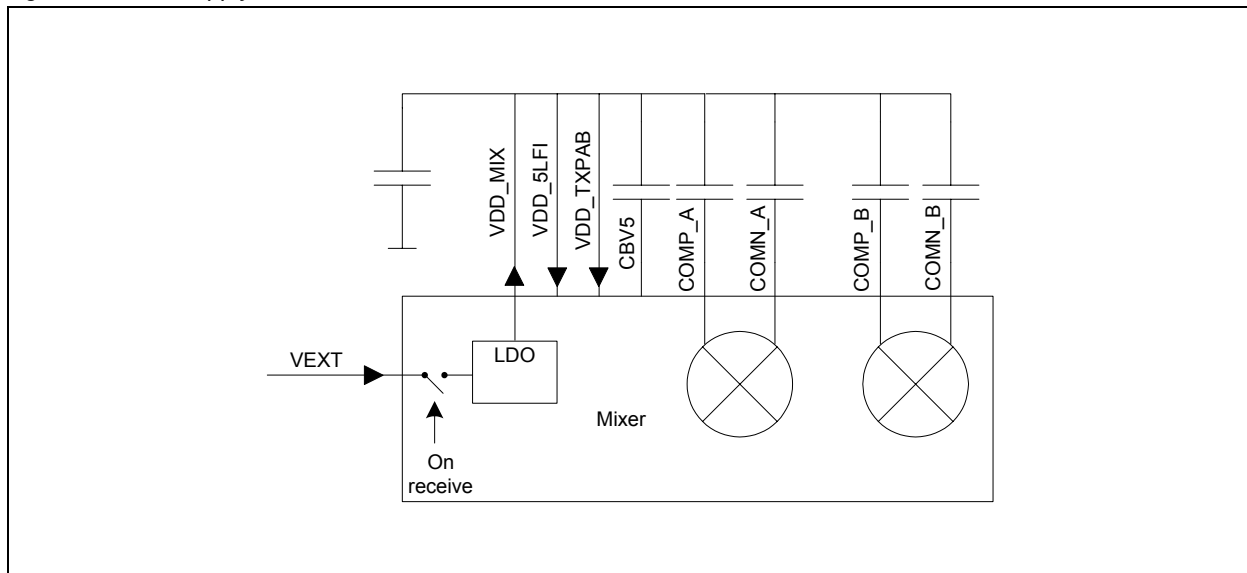
Figure 3. Mixer Supply
